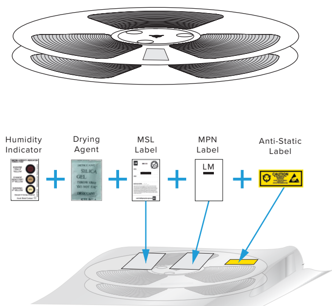
Vacuum bag.
