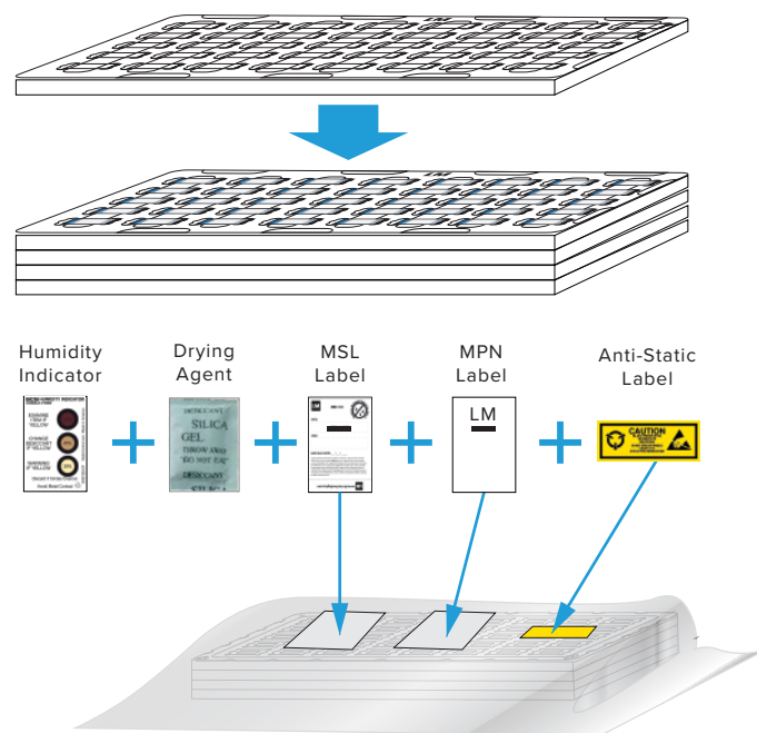
Vacuum bag.
