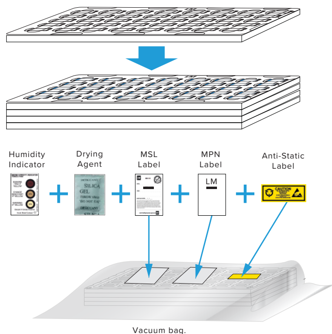
Vacuum bag.
