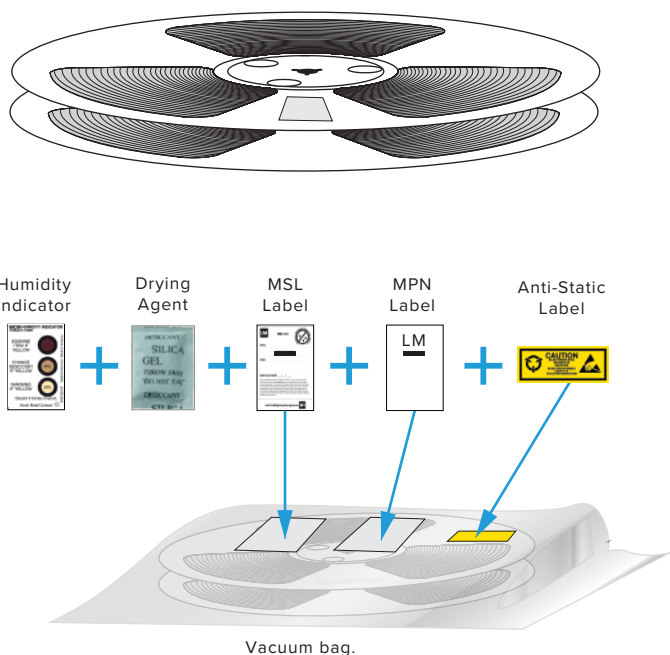
Vacuum bag.
